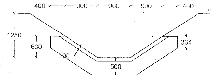
SECTION F - F
