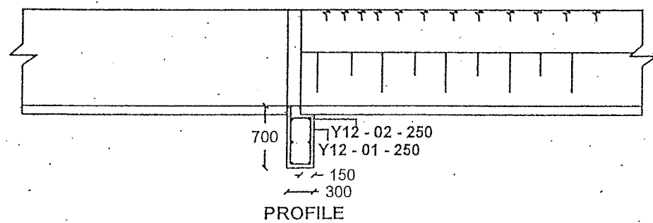
REINFORCEMENT DETAIL
