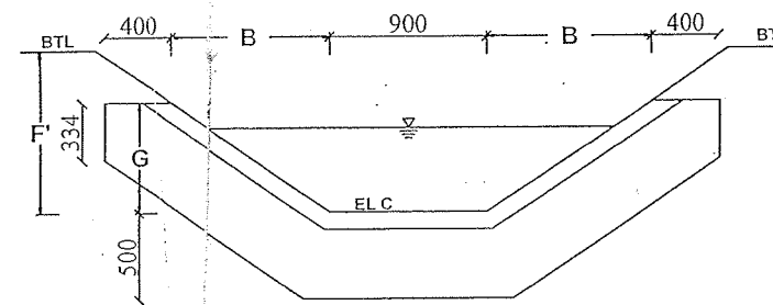
SECTION F - F
