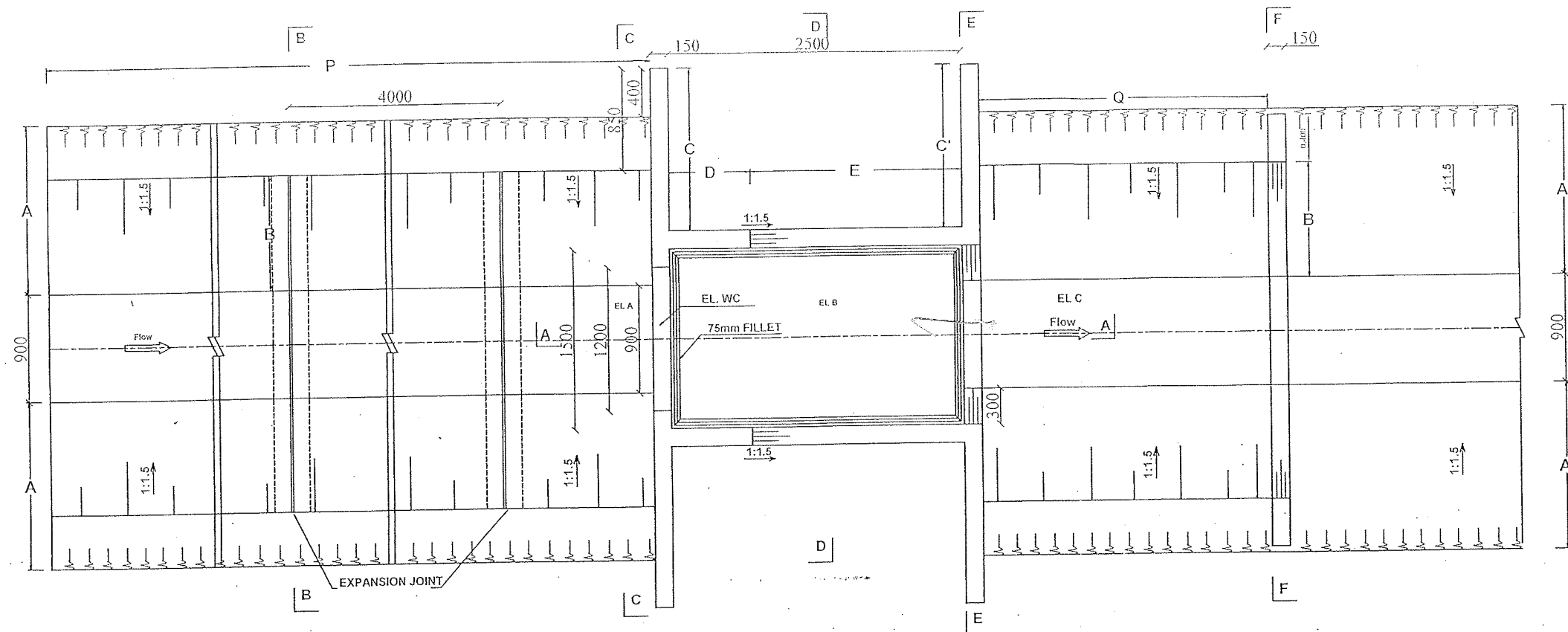
PLAN TYPICAL VERTICAL DROP STRUCTURE
