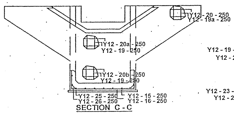
REINFORCEMENT DETAIL
