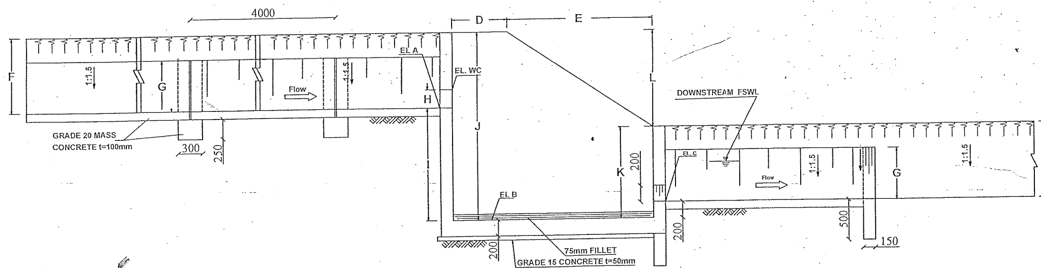
PROFILE TYPICAL VERTICAL DROP STRUCTURE
