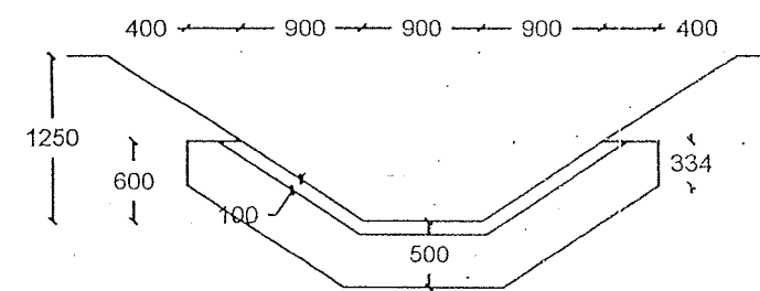
SECTION F - F
