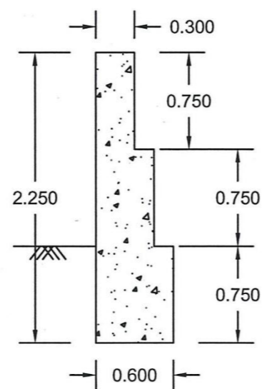
2+200 Drop D/S Retaining Wall Section
