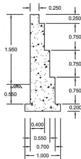
SECTION B-B
