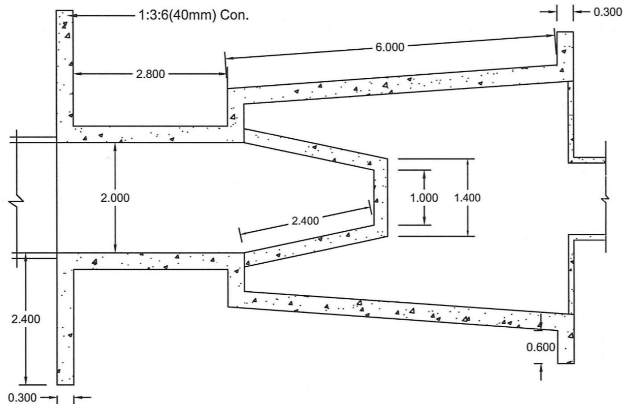
PLAN 2+200 Drop Structure
