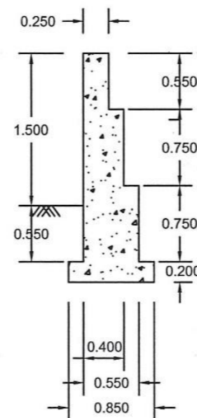
SECTION C-C
