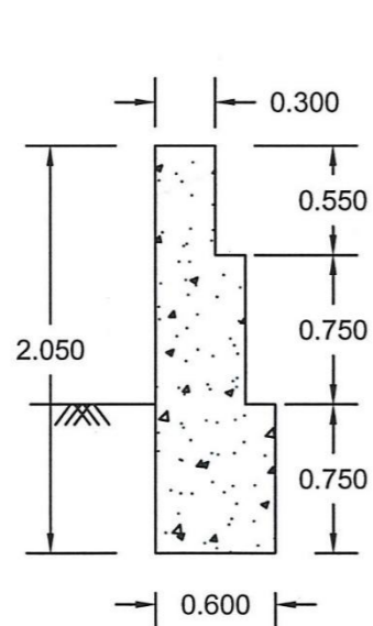
2+200 Drop U/S Retaining Wall Section
