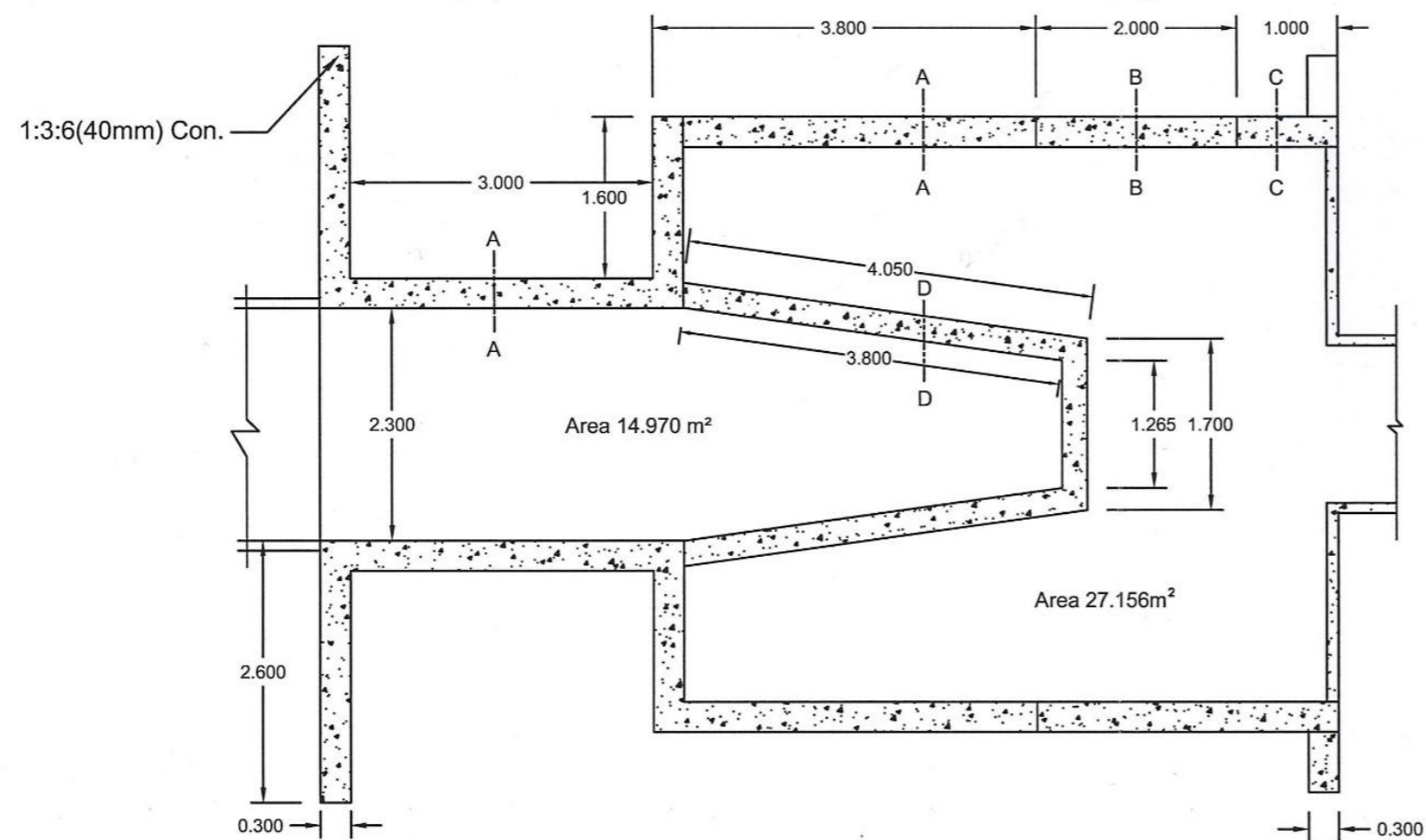
PLAN 1+500 Drop Structure
