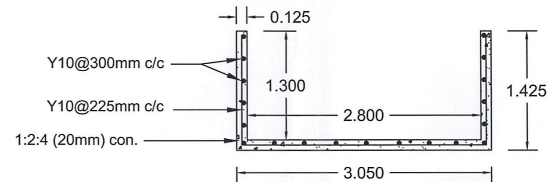
Section For Lining
