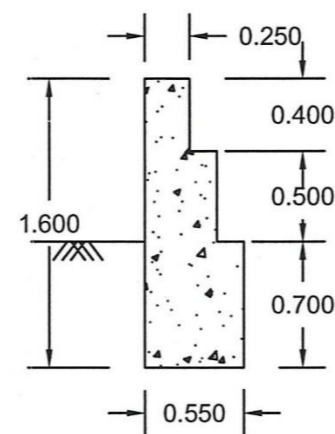
2+200 Drop Hump Section
